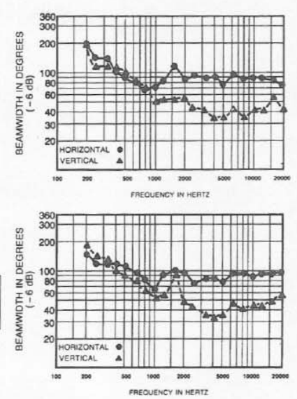
FIGURE 3 MTH-2/94A Beamwidth vs. Frequency
